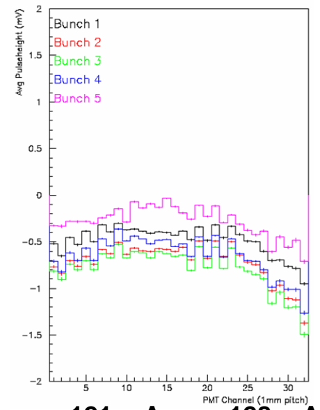
e+ = 121 mA, e- = 128 mA (0729)
