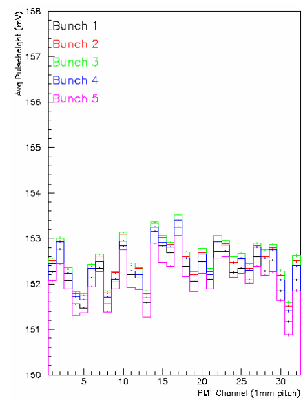
e+ = 121 mA, e- = 128 mA (0729)
