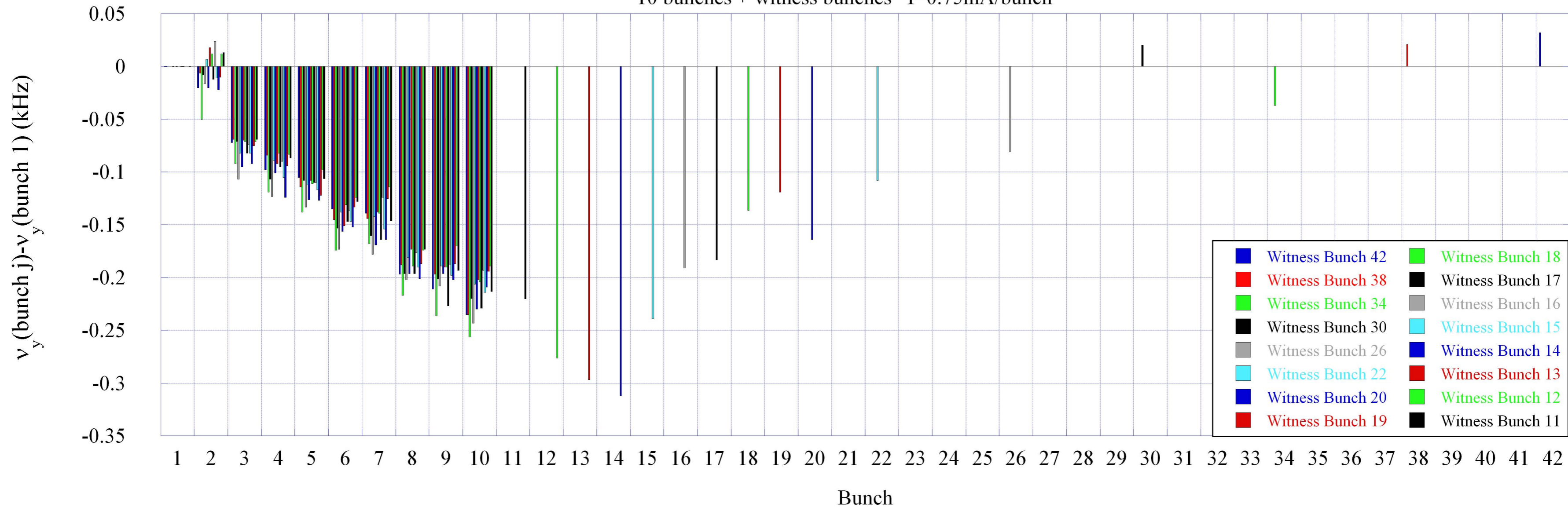
e- Vertical Tune 10 bunches + witness bunches I=0.75mA/bunch
