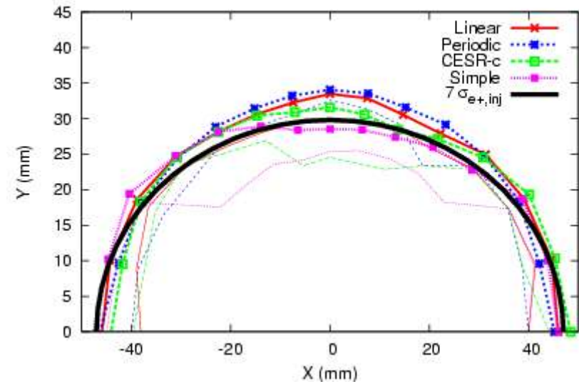
OCS for RDR, Multipole Errors, 15 Seeds, Ave/Min
