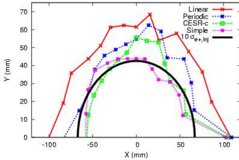
OCS for RDR, Dynamic Aperture
