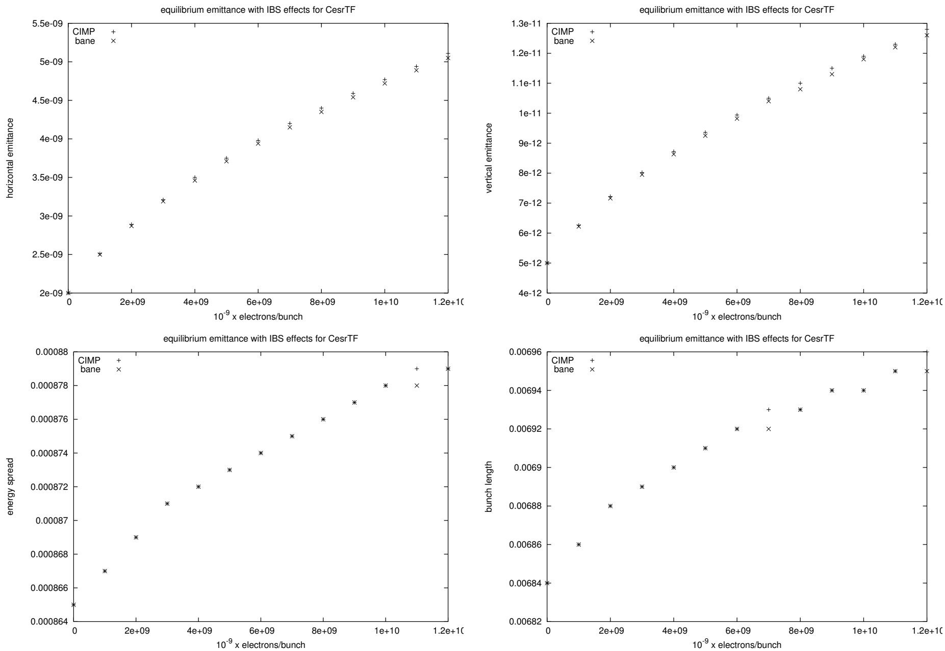
Figure 1: Equilibrium beam parameters for CesrTF as calculated in BMAD.
