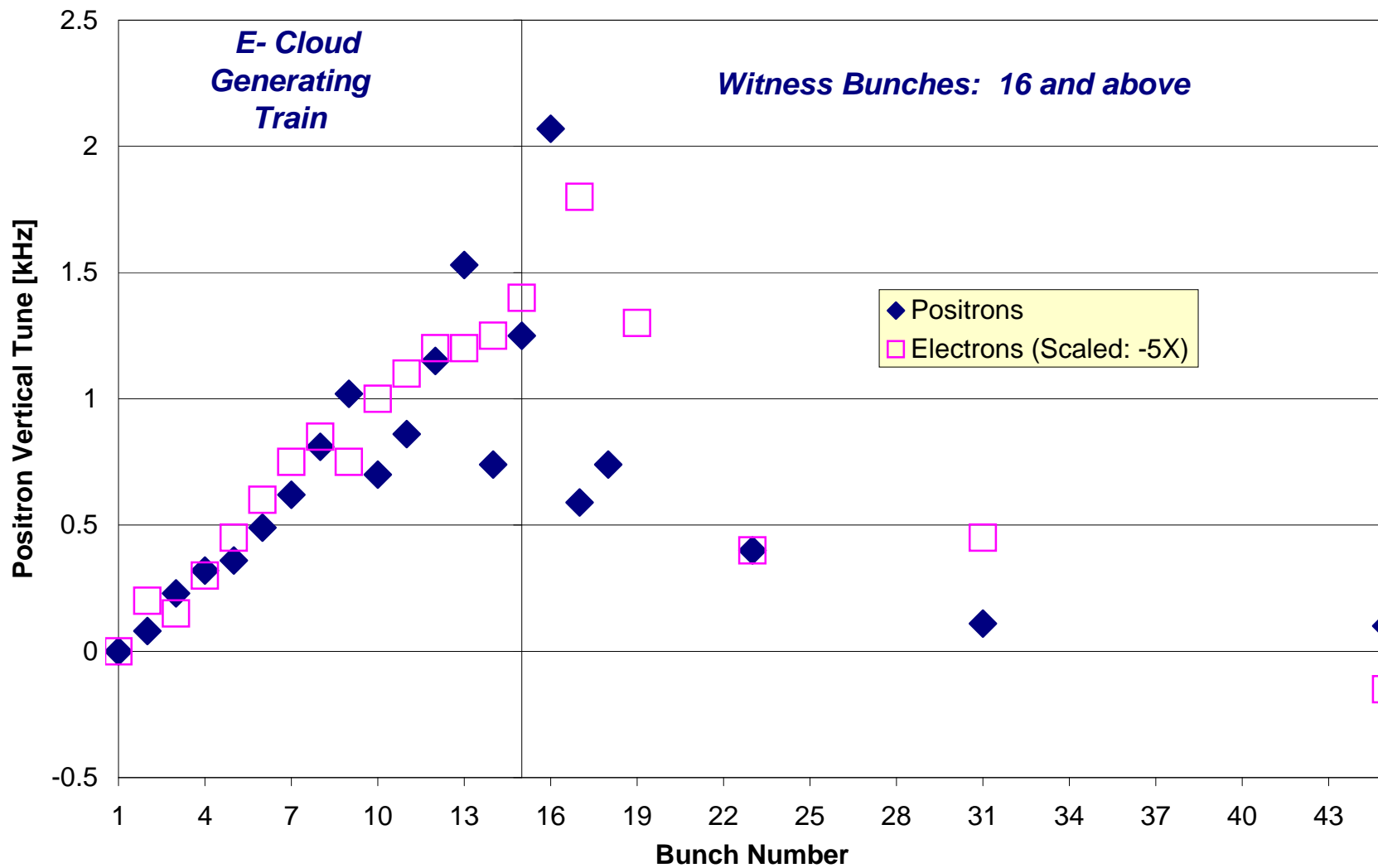
Electron-Positron Comparison with Scaled Electron Tunes
