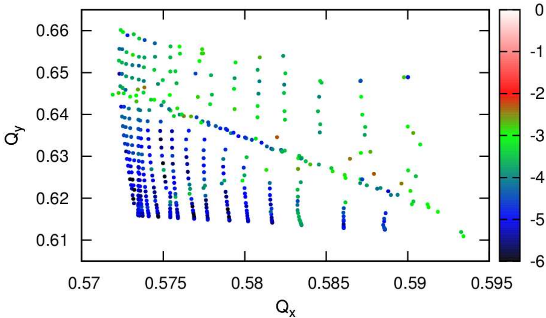
ctf-12wig-v4c-sext tune frequency map zoom
