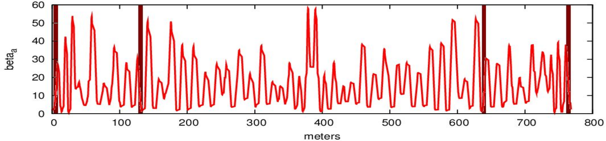
beta function for CearTA V6
