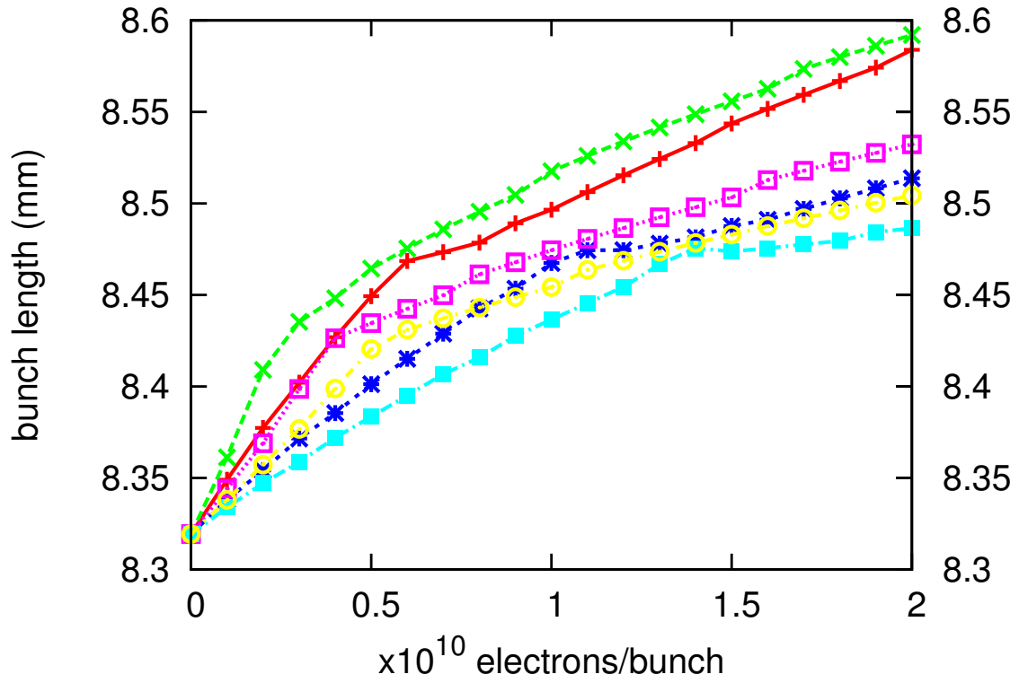
IBS Bunch Length Growth: 2.5 GeV V_{rf}=15 MV
