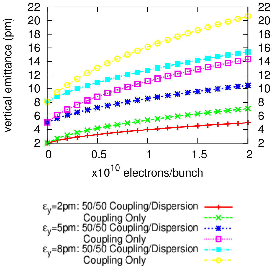
IBS Vertical Emittance Growth: 2.0 GeV V_{rf}=15 MV
