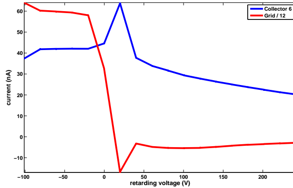
Figure 5.12: Resonant enhancement in wiggler data, 45 bunches, 1.25 mA/bunch, e+, 2.1 GeV, 14 ns. Note that there are 12 collectors, so collector 6 is one of the central ones. Also note that the grid signal is divided by 12.
