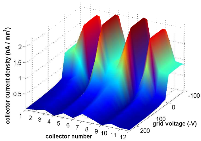
Figure 5.6: Grooved wiggler pole center RFA measurement: 1x45x1.25mA e+, 2.1GeV, 14ns
