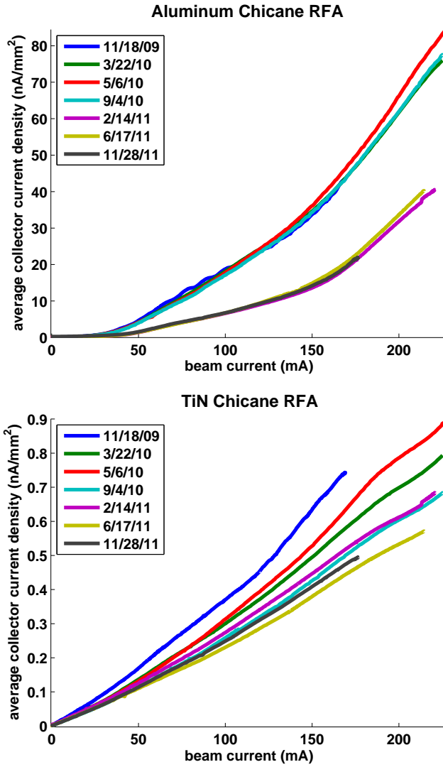
Figure 3.12: Long term behavior of chicane dipole RFAs, 1 \times 20 \text{ e}^+ , 14 ns, 5.3 GeV. Top: Aluminum chamber, bottom: TiN chamber
