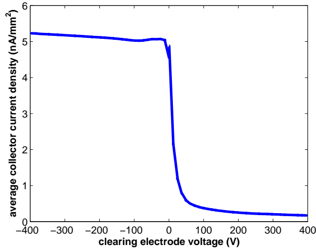
Figure 5.8: Clearing electrode scan: 1x45x1mA e+, 2.1GeV, 14ns
