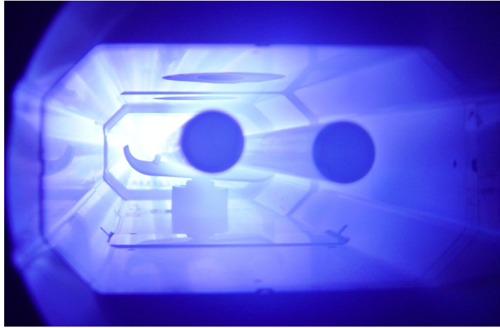
Figure 1.2: Glowing discharge during TiN coating of a CESR-TA vacuum chamber.
