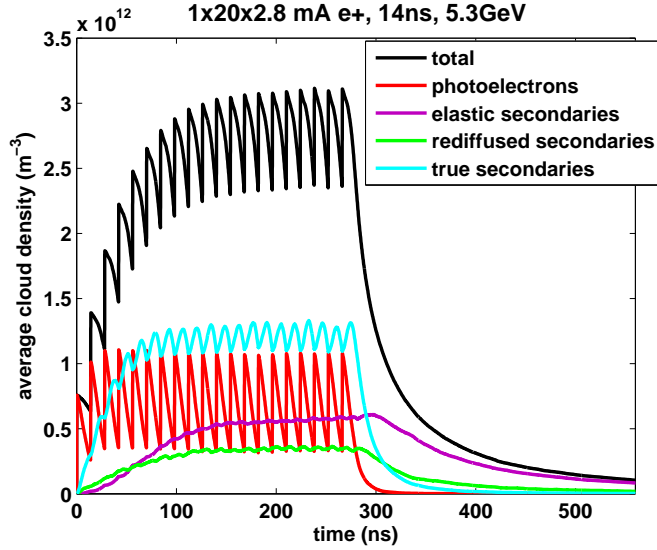
Figure 1.12: Average cloud density vs time, broken down by electron type.
