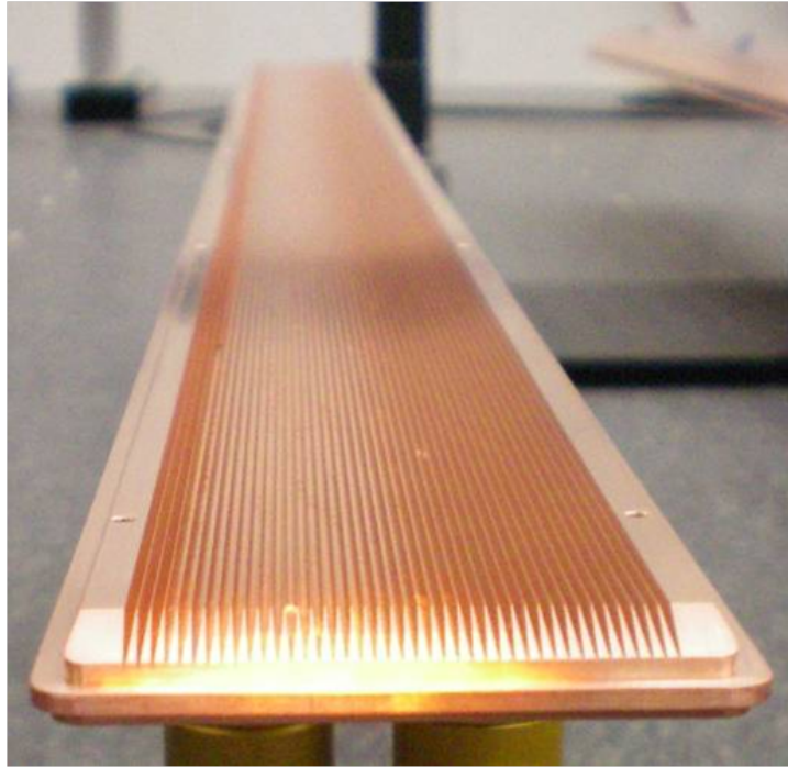
Figure 1.4: Grooved insert for CESR-TA wiggler.
