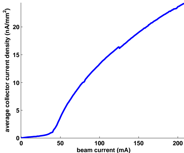
Figure 3.11: Threshold behavior in CCSR dipole RFA, 1 \times 20 e-, 5.3GeV, 14ns
