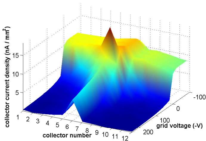
Run #2585 (1x45x1.25mA e+, 2.1GeV, 14ns): Wig1W Center Pole
