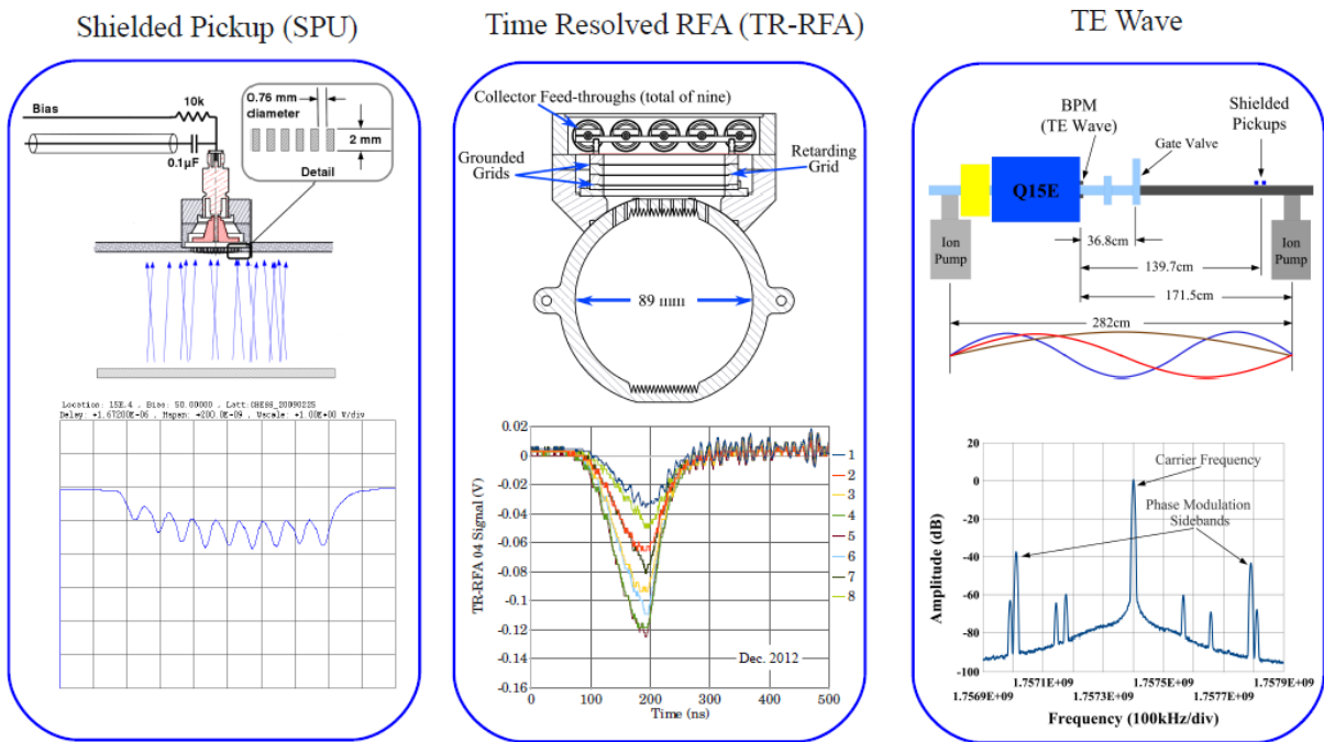
Figure 1.8: Other EC measurement techniques employed at CESR-TA .
