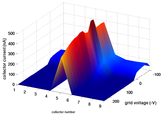
Figure 3.4: Typical Al dipole RFA voltage scans: 1 \times 45 \times 1.25 \text{ nA } e^+ , 5.3 GeV, 14 ns. Top: SLAC chicane RFA (810 Gauss); Bottom: CESR dipole RFA (2011 Gauss). In the top case, the central collector is no. 9, while in the bottom case it is no. 5.
