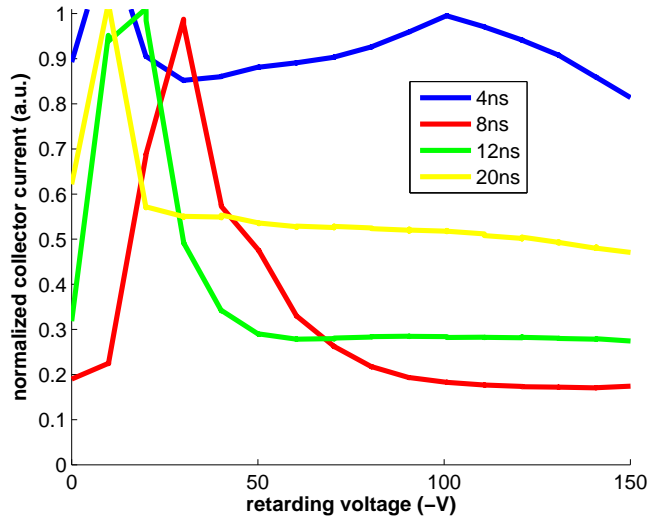
Figure 5.13: Resonant spike location at different bunch spacings, 1 \times 45 \times 1.25 mA e^+ , 5GeV. Only the signal in the central collector is plotted
