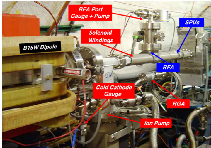
Figure 2.1: A Q15 experimental chamber installed at Q15W in CESR. In addition to the RFA, the chamber contains 4 shielded pickups (SPUs) [46].
