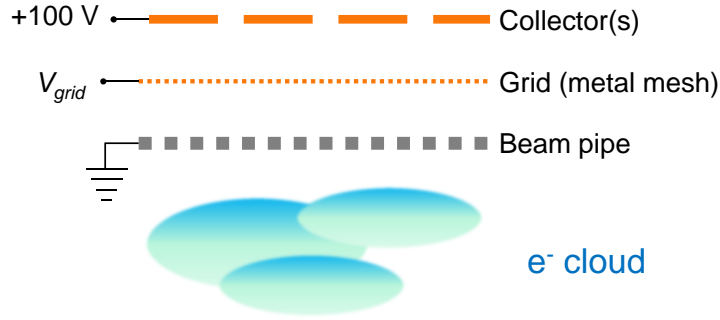
Figure 1.9: Idealized diagram of a retarding field analyzer.
