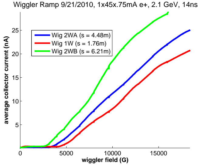
Figure 5.9: Wiggler ramp measurement: 1x45x.75mA e+, 2.1GeV, 14ns
