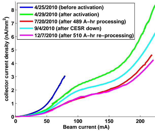
Figure 2.16: NEG RFA comparison, 1 \times 20 \text{ e}^+ , 5.3 \text{ GeV} , 14 \text{ ns}
