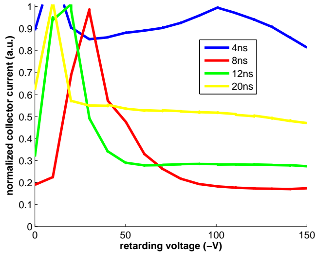
Figure 5.17: Resonant spike location at different bunch spacings, 1x45x1.25 mA e+, 5GeV. Only the signal in the central collector is plotted
