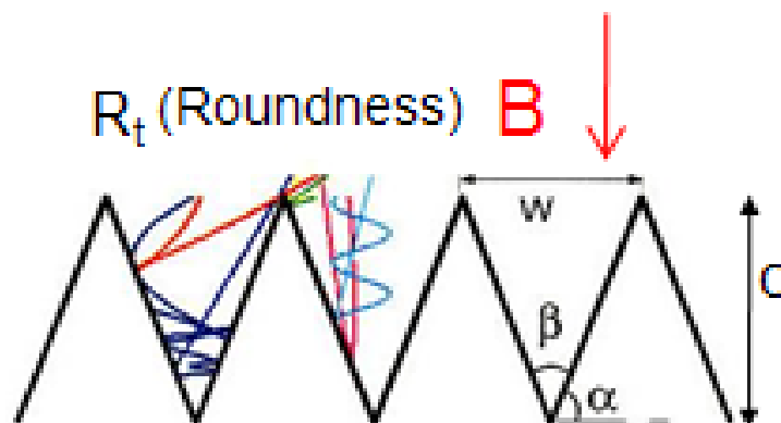
Figure 1.6: Illustration of longitudinal grooves in a dipole field, courtesy L. Wang. Important parameters in designing the grooves include the distance between peaks ( w ), groove depth ( d ), and the angle of the "valleys" ( \beta ).
