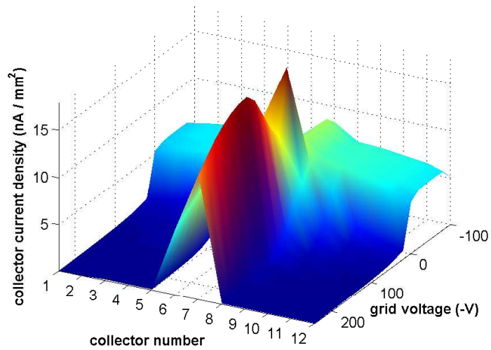
Figure 5.8: Cu wiggler intermediate field RFA measurement: 1x45x1.25mA e+, 2.1GeV, 14ns
