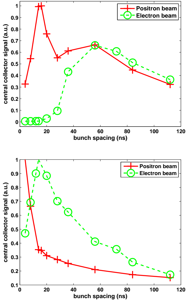
Figure 3.9: Central collector signal in a dipole RFA as a function of bunch spacing, for a 20 bunch train with 3.5mA ( 5.6 \times 10^{10} particles) per bunch, at 5.3 GeV. Top: SLAC chicane RFA, bottom: CESR dipole RFA
