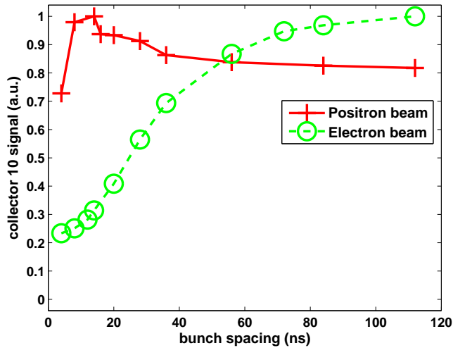
Figure 4.4: Signal in a quadrupole RFA as a function of bunch spacing, for the same beam conditions as in Fig. 3.9. The collector which is in line with the quad pole tip is plotted.
