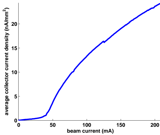
Figure 3.12: Threshold behavior in CESR dipole RFA, 1x20 e-, 5.3GeV, 14ns
