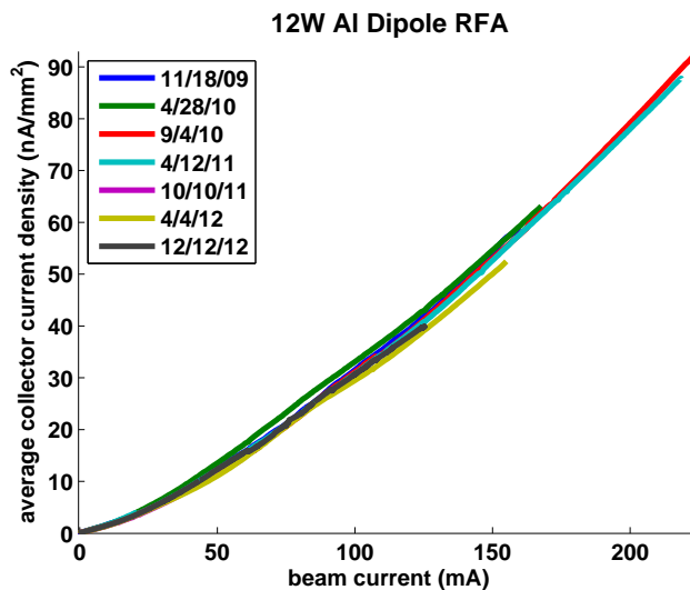
Figure 3.14: Long term behavior of CESR dipole chamber, 1 \times 20 \text{ e}^+ , 14 ns, 5.3 GeV
