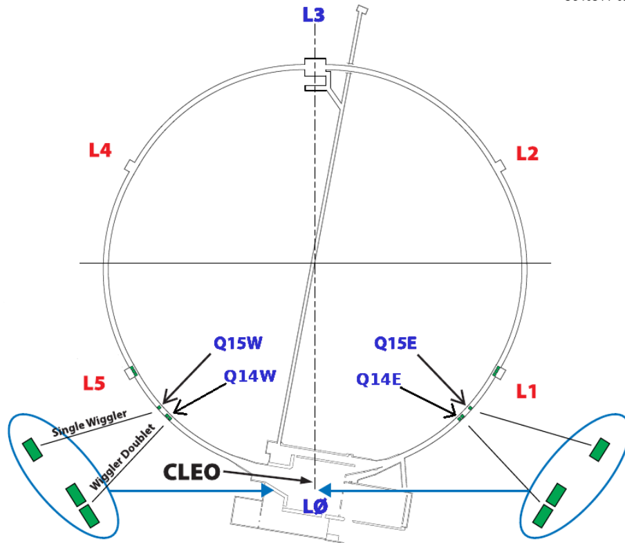
Figure 1.8: The reconfiguration of the CESR vacuum system provided space for several electron cloud experimental sections. RFAs are located at L0, Q14E/W, Q15E/W, Q19E, and L3.
