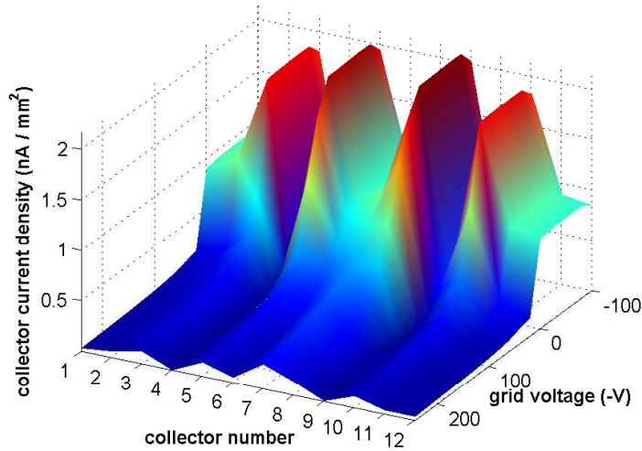
Figure 5.9: Grooved wiggler pole center RFA measurement: 1 \times 45 \times 1.25 \text{ mA } e^+ , 2.1 \text{ GeV} , 14 \text{ ns}
