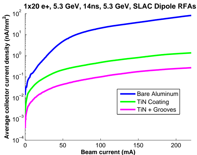
Figure 3.10: Dipole RFA mitigation comparison, 1x20 e+, 5.3GeV, 14ns, 810 Gauss.
