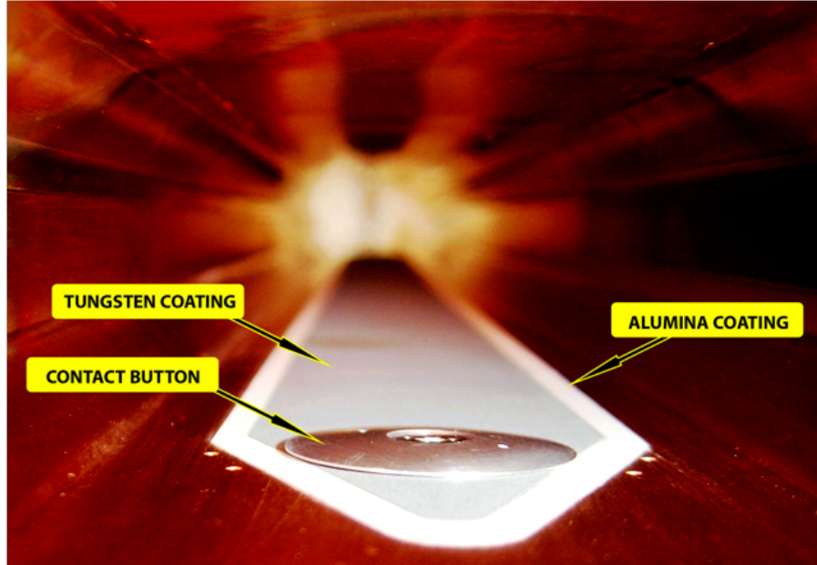
Figure 5.6: Photo of clearing electrode connection button on the bottom of a wiggler beam pipe.
