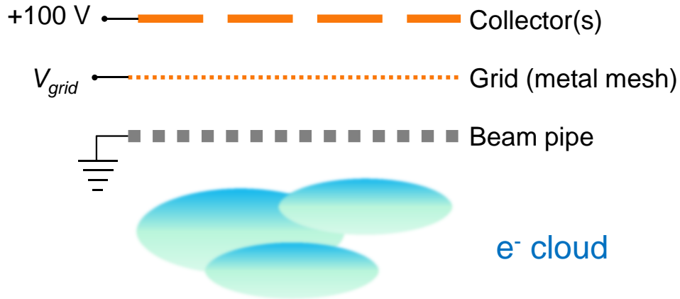
Figure 1.11: Idealized diagram of a retarding field analyzer.
