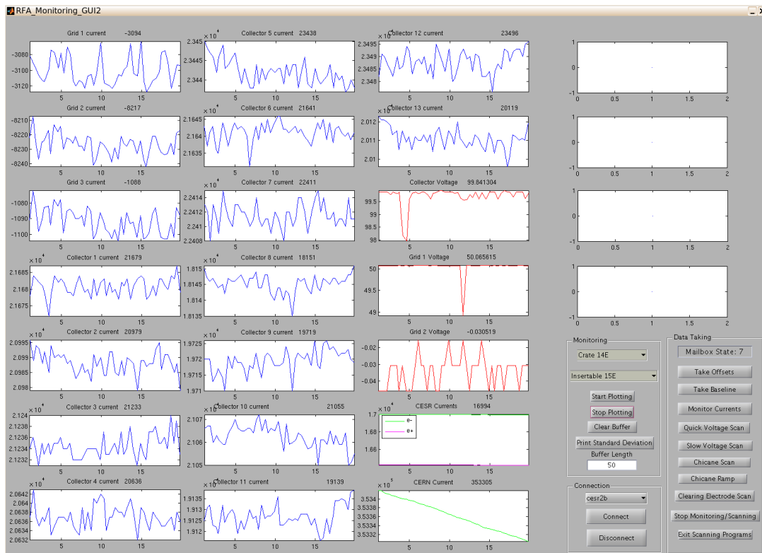
Figure 1.12: MATLAB GUI used for RFA machine studies, showing real time readout of the grid and collector currents and voltages, as well as the beam current.
