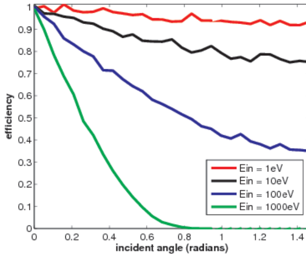
Figure 3.15: Simulated RFA efficiency vs incident angle for a SLAC chicane dipole RFA, with a .081 T magnetic field.
