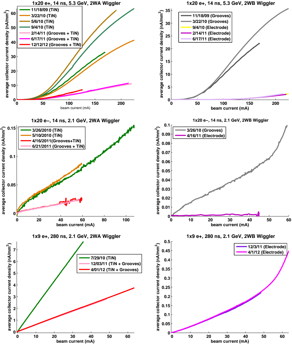
Figure A.3: Additional mitigation comparisons, L0 wiggler (center pole) RFAs. Note that the wigglers are turned off at 5.3 GeV.
