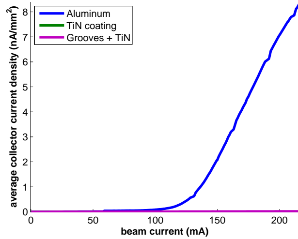
Figure 3.11: Dipole RFA mitigation comparison, 1x20 e-, 5.3GeV, 14ns, 810 Gauss.
