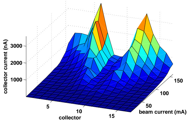
Figure 3.17: Simulation of the bifurcation of peak cloud density: 1 \times 10^{20} e+, 5.3 GeV, 14 ns. Compare to Fig. 3.6
