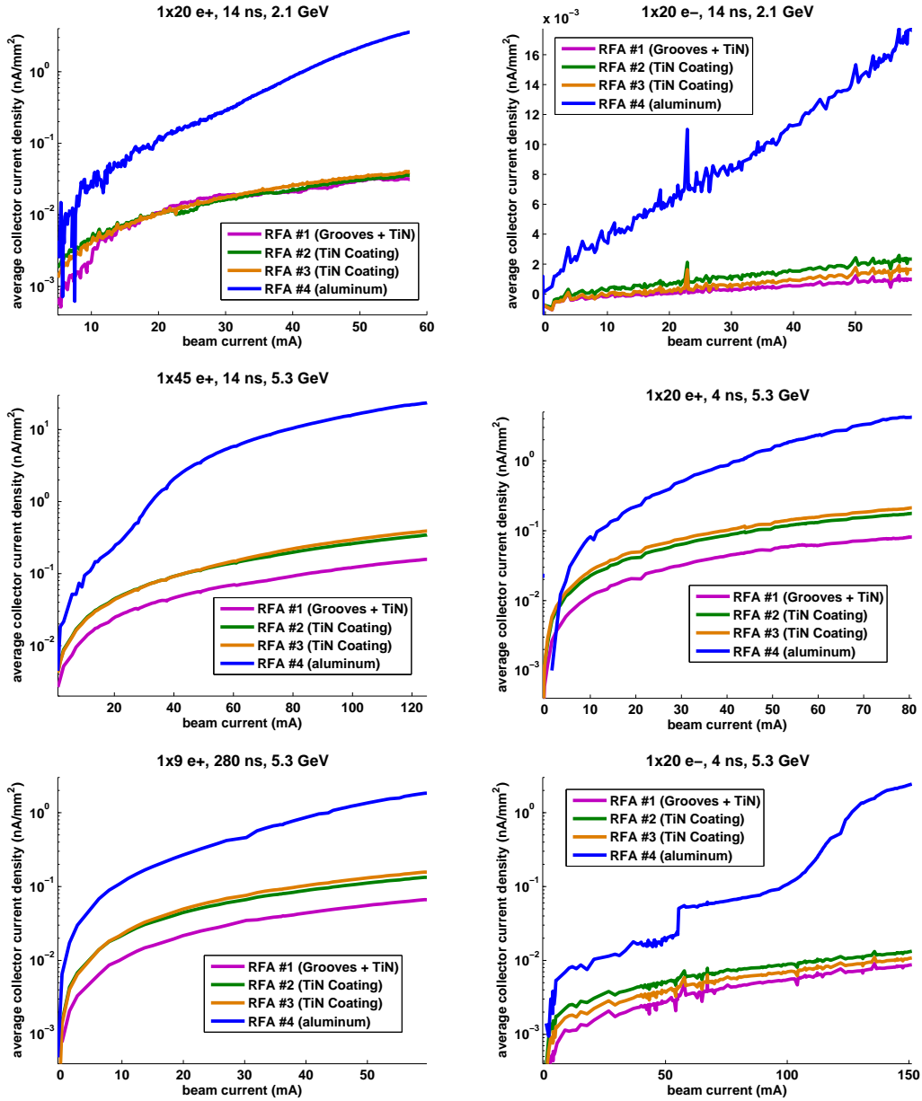
Figure A.2: Additional mitigation comparisons, chicane dipole RFAs
