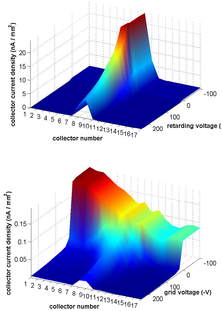
Figure 3.5: Chicane dipole RFA voltage scans: 1 \times 45 \times 1.25 mA e+, 14 ns, 5.3 GeV, 810 Gauss. Top: Aluminum chamber; Bottom: TiN-coated chamber. The central collector is no. 9.
