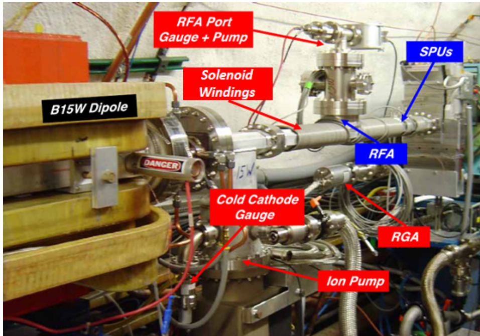
Figure 2.1: A Q15 experimental chamber installed at Q15W in CESR. In addition to the RFA, the chamber contains 4 shielded pickups (SPUs) [64].
