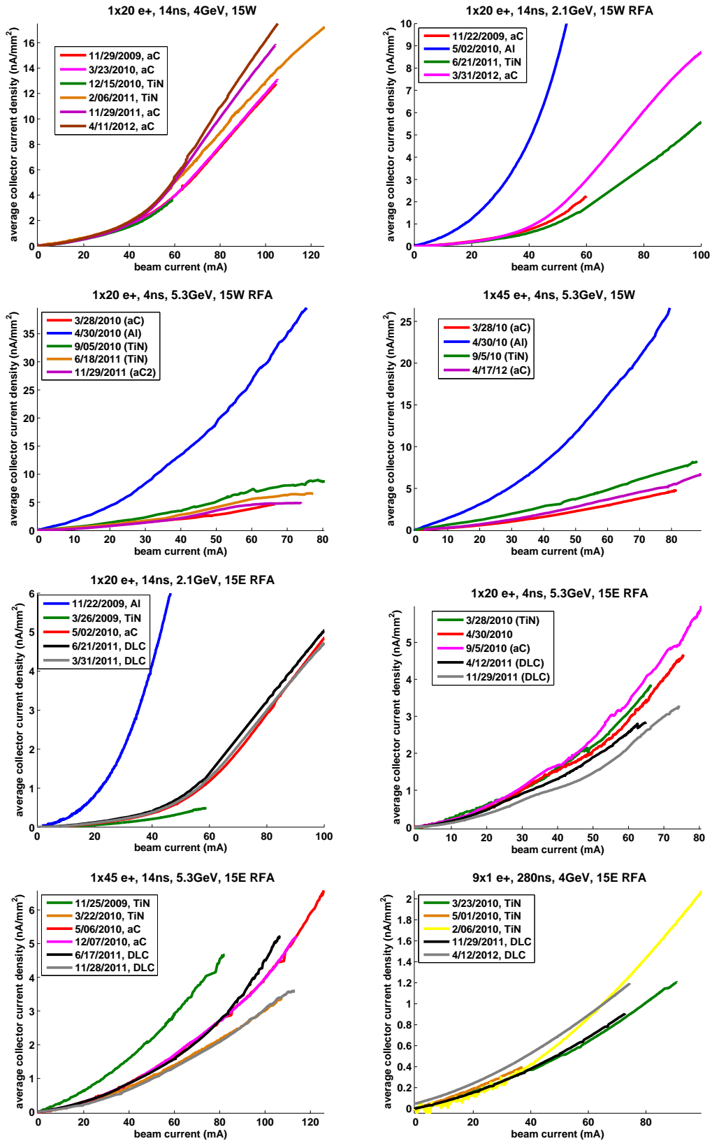
Figure A.1: Additional mitigation comparisons, 15E/W drift RFAs
