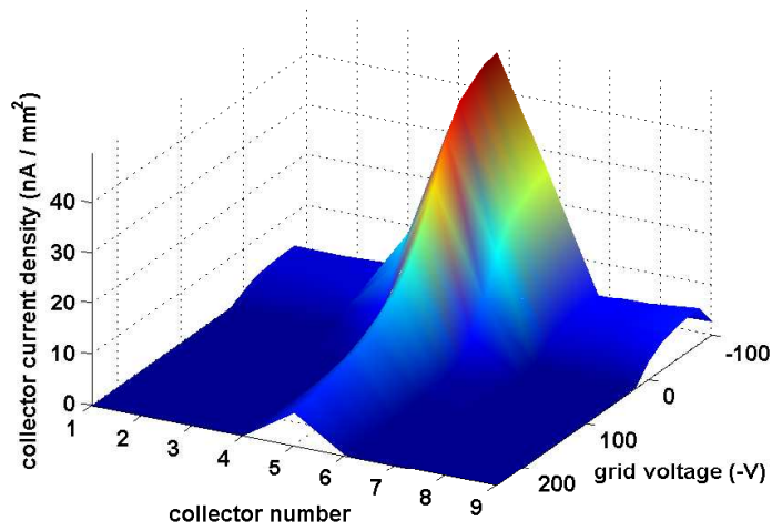
Figure 3.4: CESR dipole RFA voltage scans: 1 \times 45 \times 1.25 \text{ mA } e^+ , 14ns. Top: 5.3 GeV (2010 Gauss); Bottom: 2.1 GeV (790 Gauss). The central collector is no. 5, and the chamber is made of uncoated aluminum.
