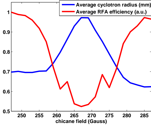
Figure 3.19: Effect of cyclotron resonance on RFA efficiency, 1x45x1 mA e+, 4 ns, 5 GeV. Under the resonant field, the average electron cyclotron radius increases, resulting in a decrease in the average RFA efficiency.
