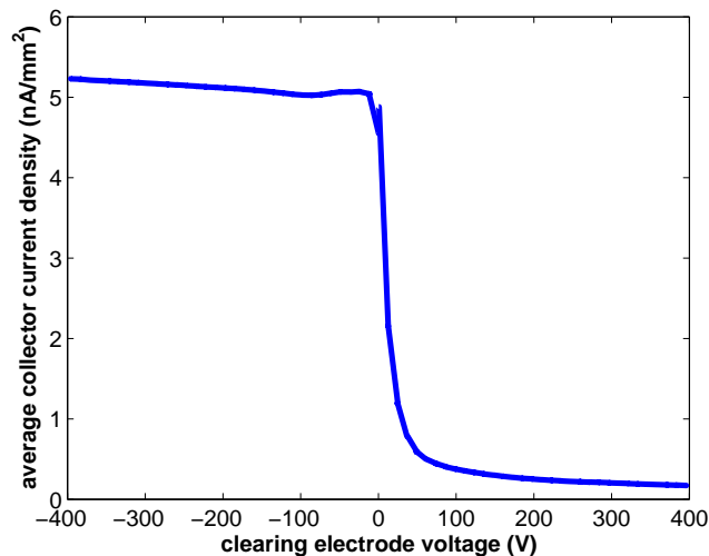
Figure 5.11: Clearing electrode scan: 1x45x1mA e+, 2.1GeV, 14ns
