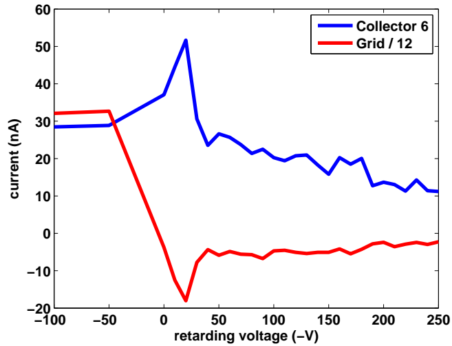
Figure 5.18: POSINST simulation showing resonant enhancement, 1 \times 45 \times 1.2 mA e+, 2.1 GeV, 14 ns, central collector. Compare to Fig. 5.16.
