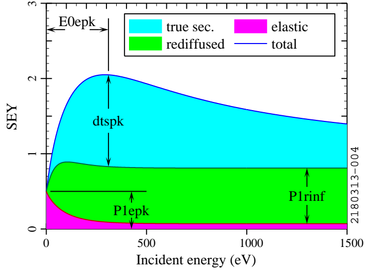
Figure 1.13: The POSINST model for secondary electron yield as a function of energy, with important parameters indicated.
