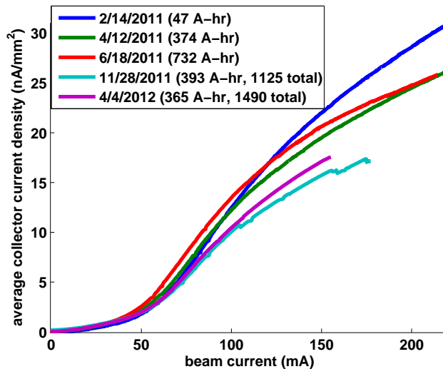
Figure 2.15: Performance of Q15E DLC chamber over time, 1 \times 20 e^+ , 5.3 GeV, 14 ns. Integrated beam doses are given for each measurement. Where two doses are shown, the first is counted from the last CESR down, and the second from the installation of the chamber.
