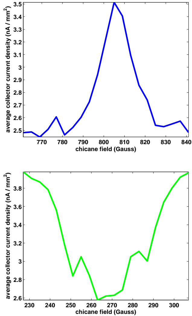
Figure 3.18: Simulation of cyclotron resonances observed by an RFA in aluminum (top) and TiN (bottom) chambers, 1x45x1 mA e+, 4 ns, 5 GeV. Note that, as in Fig. 3.8, the resonance appears as an increase in the aluminum chamber signal, but a decrease in the TiN chamber signal.
