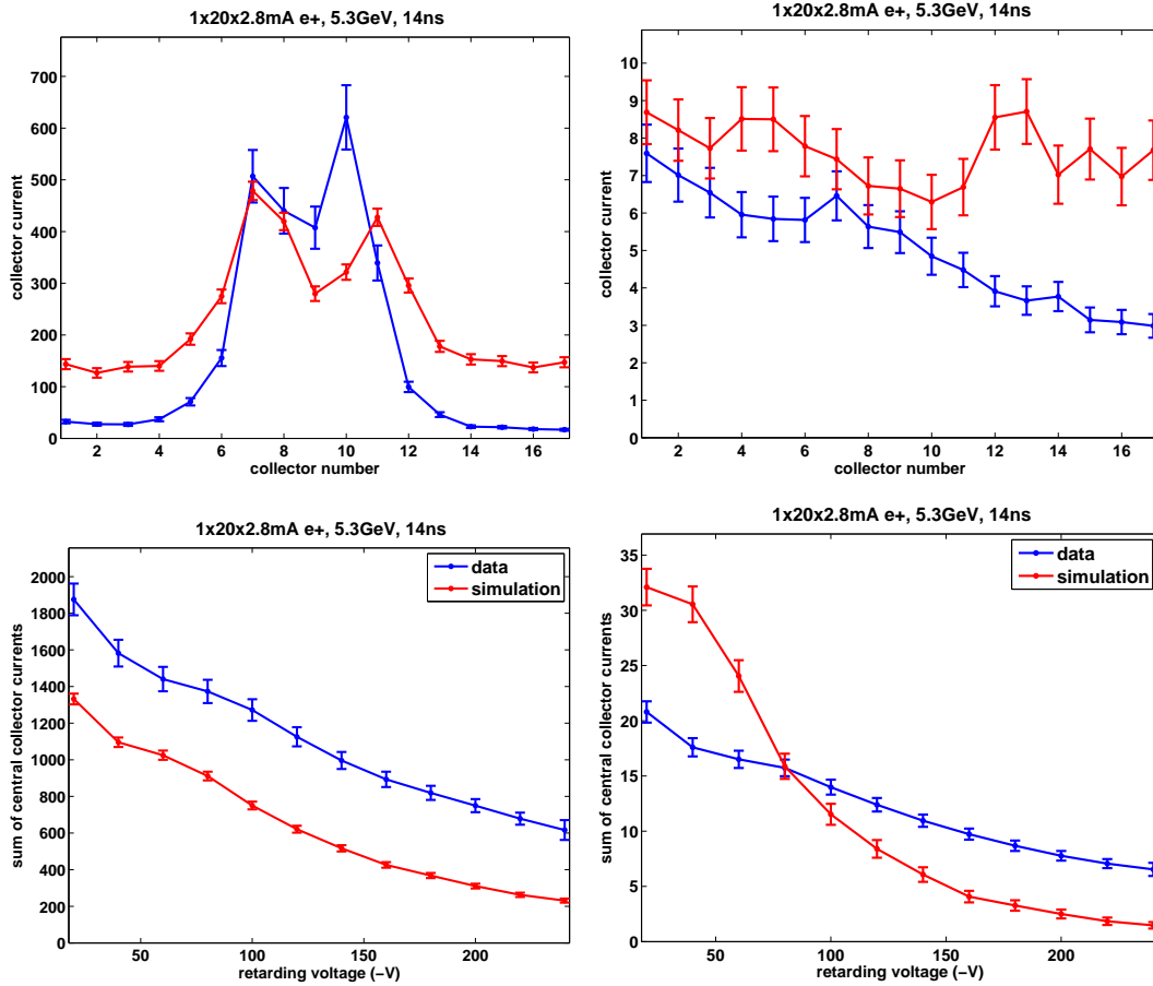
Figure 3.16: Comparison of chicane RFA data and simulation, using best fit parameters for aluminum (left, see Table 2.6), and TiN (right, see Table 2.8). The top plots show the total signal across the 17 RFA collectors (with +50 V on the grid); the bottom plots show the signal in the central five collectors vs retarding voltage.
