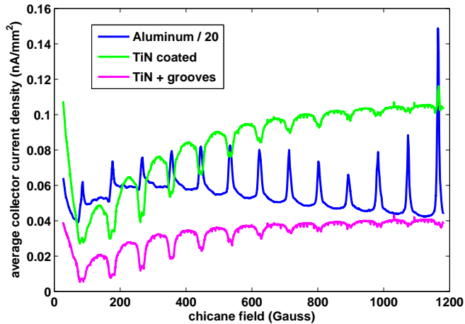
Figure 3.8: RFA signal as a function of chicane magnetic field: 1x45x1 mA e+, 5 GeV, 4 ns. Cyclotron resonances are observed every 89 G. Note that the Aluminum chamber signal is divided by 20.
