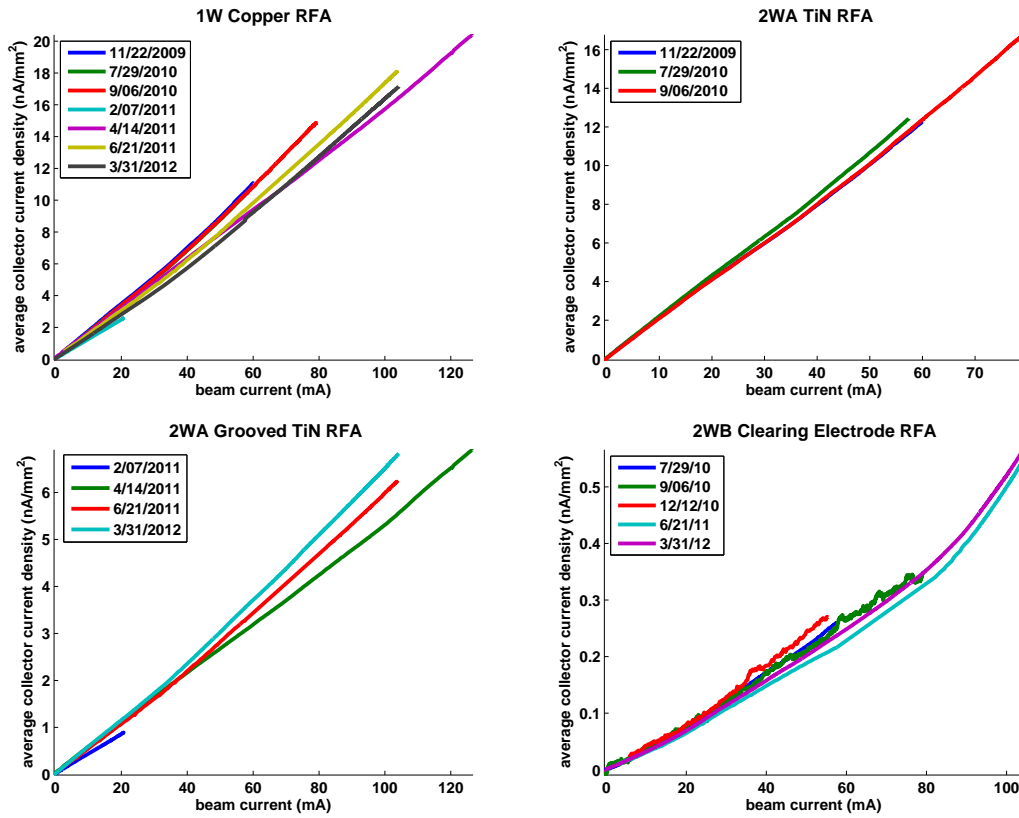
Figure 5.15: Long term behavior of wiggler chambers: 1x20 e+, 2.1GeV, 14ns. Top left: 1W Copper chamber; top right 2WA TiN chamber; bottom left: 2WA grooved TiN chamber; bottom right: 2WB clearing electrode chamber.
