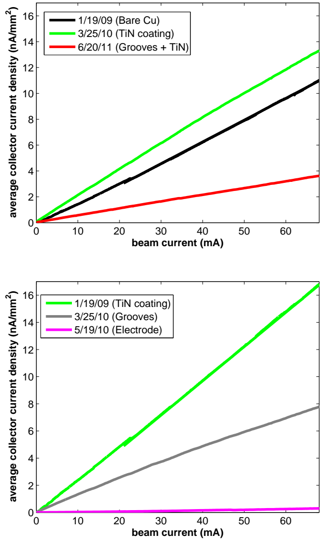
Figure 5.14: Wiggler RFA mitigation comparison: 1 \times 45 e+, 2.1 GeV, 14 ns. Top: 2WA location, bottom: 2WB location. The 2WB location is further downstream in the wiggler straight, and therefore has a slightly higher photon flux.
