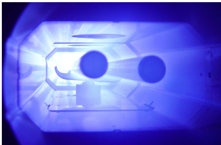
Figure 1.4: Glowing discharge during TiN coating of a CESR-TA vacuum chamber.
