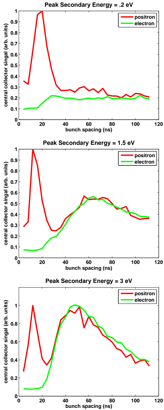
Figure 3.20: Simulation of the multipacting resonances: 1 \times 20 \times 3.5 mA, 5.3 GeV, for different “true secondary” energies. Top: E_{ts} = .2 eV, middle: E_{ts} = 1.5 eV, bottom: E_{ts} = 3 eV. The locations of the resonances are very sensitive to this parameter. Compare to Fig. 3.9.
