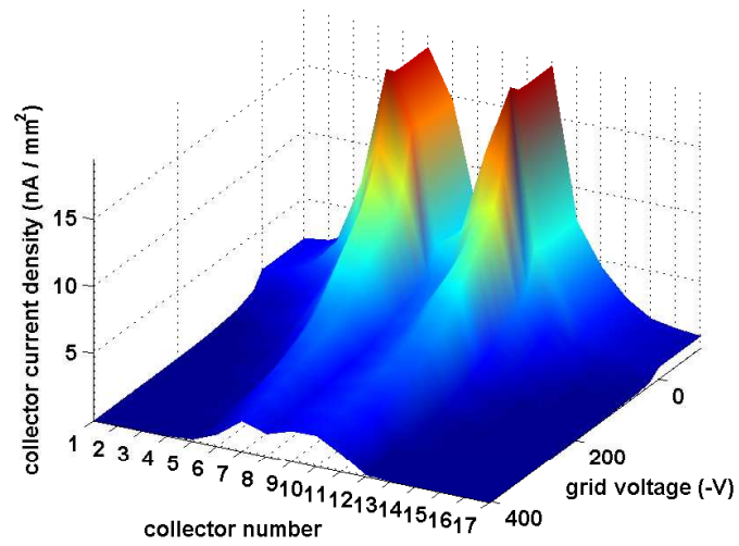
Figure 3.7: Chicane RFA voltage scan at high beam current: 1x20x5 mA e+, 5.3 GeV, 14 ns. Bifurcation is clearly visible
