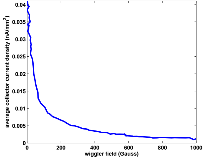
Figure 5.13: Wiggler ramp measurement in longitudinal field region: 1x45x.75mA e+, 2.1GeV, 14ns
