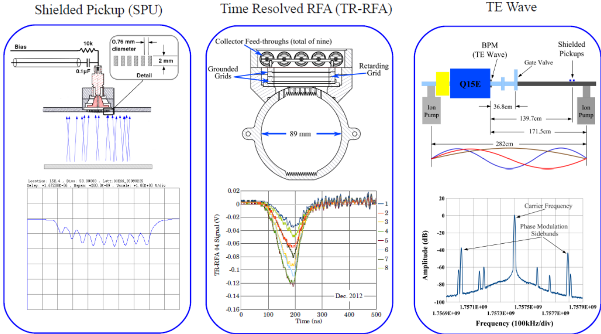
Figure 1.9: Other EC measurement techniques employed at CESR-TA , courtesy J. Sikora.
