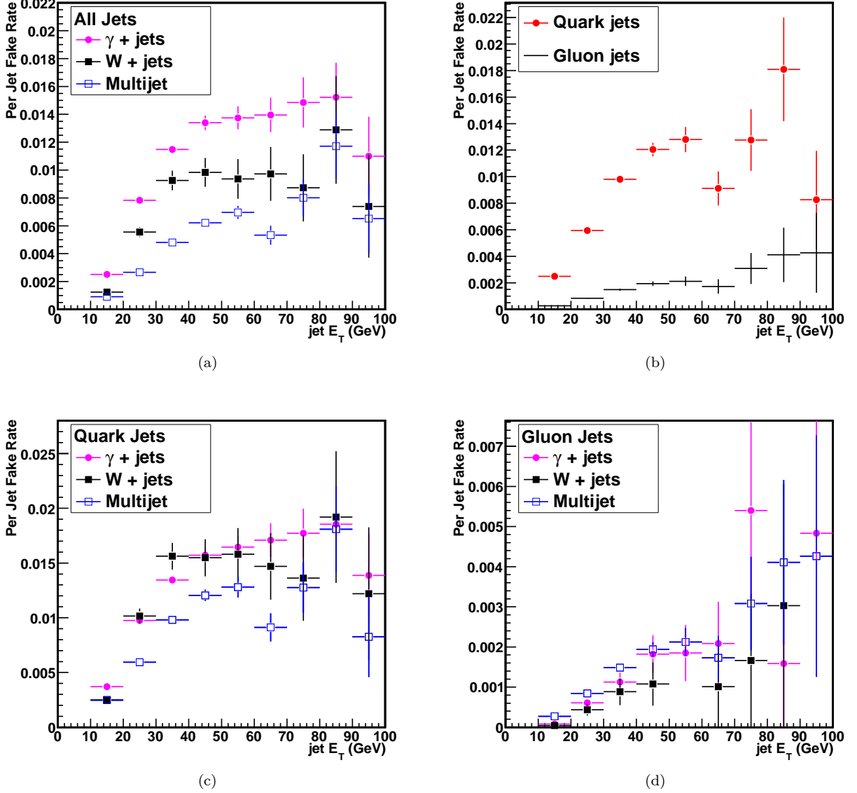
FIG. 6: Track lepton fake rates in simulation as a function of denominator jet E_T . (a) Fake rate for all jets in simulated \gamma + \text{jets} , W + \text{jets} , and multijet events. The fake rate in multijet events is lower than the fake rate in W + \text{jets} events, and both are lower than that in \gamma + \text{jets} events. Note that this \gamma + \text{jets} sample does not have the E_\gamma > 80 GeV requirement applied. (b) Fake rate for jets matched to quarks (“quark jets”) compared to the fake rate for jets matched to gluons (“gluon jets”), showing the disagreement between them. Fake rates taken from the simulated multijet sample. (c) Fake rates for quark jets in the three samples. The agreement is better than that observed in (a). (d) The same, but for jets matched to gluons.
