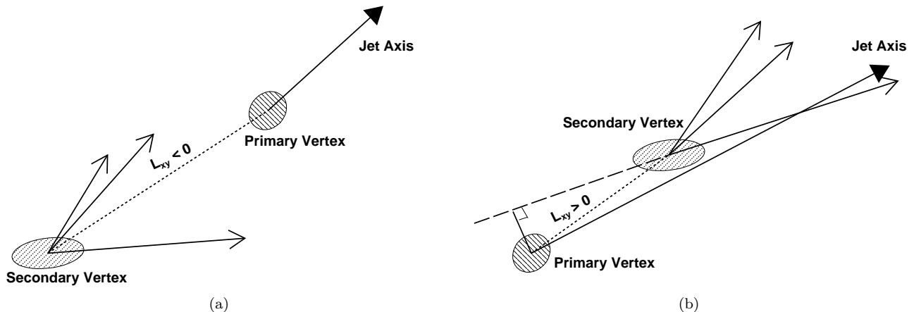
FIG. 3: Drawing showing reconstructed secondary vertices, illustrating example cases where (a) L_{xy} < 0 and (b) L_{xy} > 0 .
