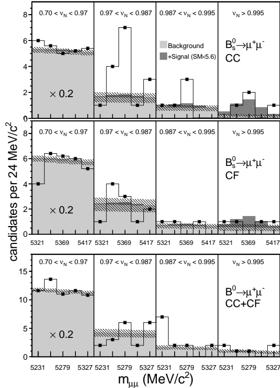
FIG. 1: The observed number of events (open histogram with points) is compared to the total expected background (light grey) and its uncertainty (hatched) in bins of dimuon invariant mass. The top and middle rows show the results in the B_s^0 mass signal region for the CC and CF channels, respectively. The bottom row shows the results in the B^0 mass signal region for the CC and CF channels combined. The results for the first 5 \nu_N bins are combined (and scaled by 0.2) while the results for the last three bins are each shown separately. Also shown is the expected contribution from B_s^0 \rightarrow \mu^+\mu^- events (dark gray) using the fitted branching fraction, which is 5.6 times the expected SM value.
